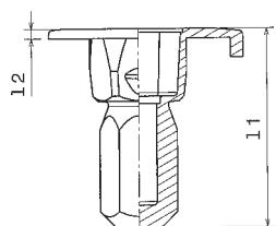
K' in K' bottom part screw-in blind rivet
