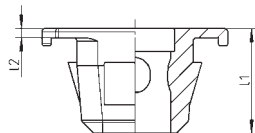
K' in K' bottom part spread nut
